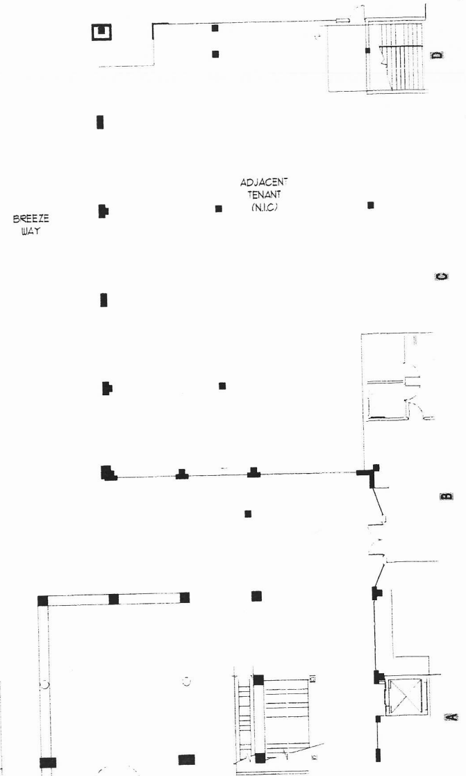
1 DEMISING PLAN 1/8" = 1'-0"
